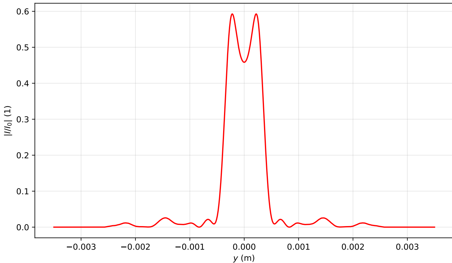
Intensity profile I(x = 0, y, z = 0.637)/I_0 , P_{in}=4.0P_{cr} , artificial time
